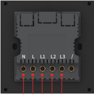
N L L1 L2 L3 / Power cord socket Load power cord socket
