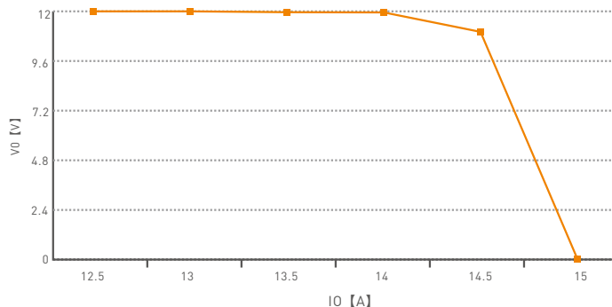
Over Load Diagram
